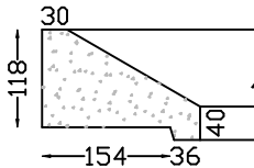
WINDOW SILL TYPE 13 Variable length max 1,900m
