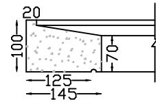
WINDOW SILL TYPE 12 Variable length max 1,500m
