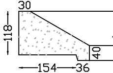
WINDOW SILL TYPE 13 Variable length max 1,900m
