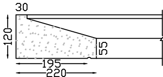
WINDOW SILL TYPE 10 Variable length max 1,500m
