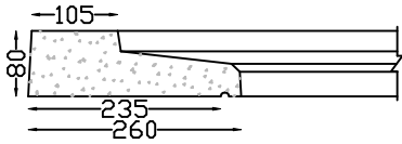
WINDOW SILL TYPE 1 Length 1,200m
