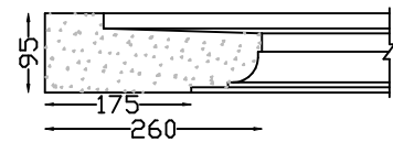
WINDOW SILL TYPE 9 Length 1,350m max
