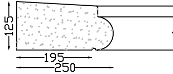
WINDOW SILL TYPE 5 Length 1,200m
