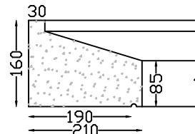
WINDOW SILL TYPE 15 Length 1100mm
