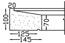
WINDOW SILL TYPE 12 Variable length max 1,500m
