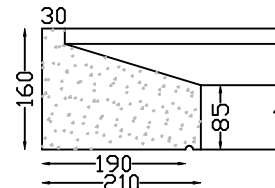
WINDOW SILL TYPE 15 Length 1100mm
