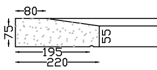
WINDOW SILL TYPE 11 Variable length max 2,000m
