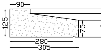
WINDOW SILL TYPE 14 Variable length max 1,160m
