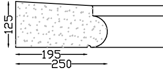
WINDOW SILL TYPE 5 Length 1,200m
