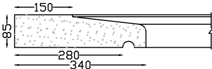
WINDOW SILL TYPE 6 Length 1,200m
