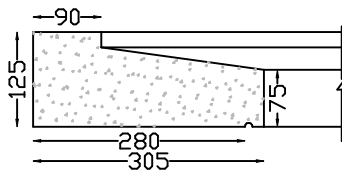
WINDOW SILL TYPE 14 Variable length max 1,160m
