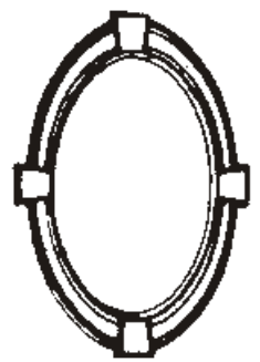
KEYSTONE ELIPSE MAJOR 1,860m x 1,180m MINOR 1,260m x 850mm
