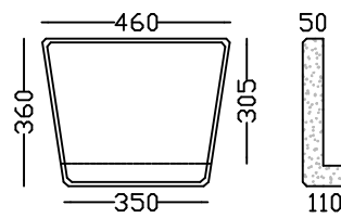
KEYSTONE VENEER 360
