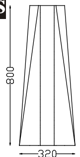
800mm high x 320/200mm Hole 80mm
