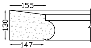
WINDOW SILL TYPE 3 Length 1,200m
