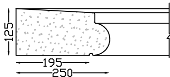
WINDOW SILL TYPE 5 Length 1,200m. Corner. Curve
