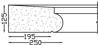
WINDOW SILL TYPE 5 Length 1,200m. Corner. Curve
