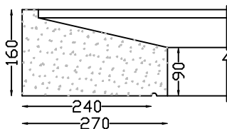
WINDOW SILL TYPE 20 Length 1,200m max
