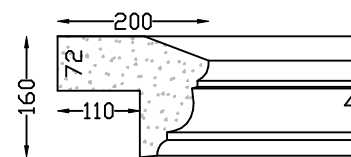
WB REBATE SILL Max 2,000m long with L and R returns (in one piece). Greater lengths in more than one piece.
