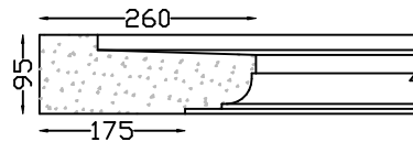
WINDOW SILL TYPE 9 Length 1,350m Max
