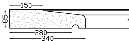
WINDOW SILL TYPE 6 Length 1,150m
