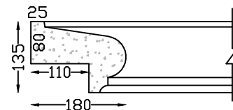
BULLNOSED SILL Max 1,600m sill opening width, with L and R returns (in one piece). Greater lengths in more than one piece.
