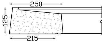
WINDOW SILL TYPE 2 Length 1,750m Max
