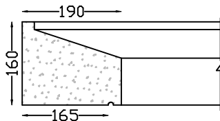
WINDOW SILL TYPE 4 Length 1,200m
