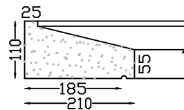
WINDOW SILL TYPE 16 Length 1,500m Max
