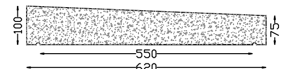
DRIPSTONE 550 "B" COPING Length 750mm
