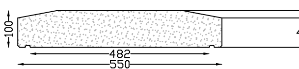
ILOVO 550/480 COPING Length 600mm
