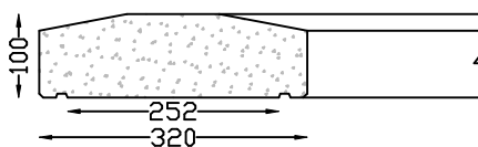
ILOVO 320/250 COPING Length 620mm
