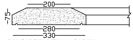
PALISADE PLINTH 330 COPING Length 800mm
