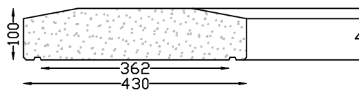
ILOVO 430/360 COPING Length 600mm
