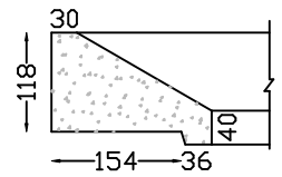
WINDOW SILL TYPE 13 Length: Max 1,900m
