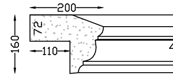
WB REBATE SILL
