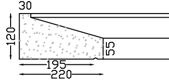
WINDOW SILL TYPE 10 Length: 1,500m Max
